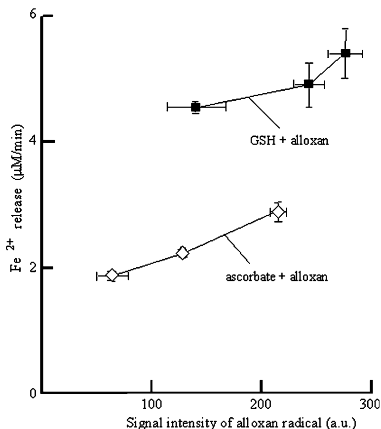
Figure 6. Iron release from ferritin as a function of A^{\cdot -} signal intensity. Iron release was measured under the conditions described in Figures 1 and 5b except that the concentration of alloxan varied from 1 to 3 mM. The generation of the alloxan radical was determined by ESR spectrometry. Each value represents the mean \pm S.D. of three experiments.
