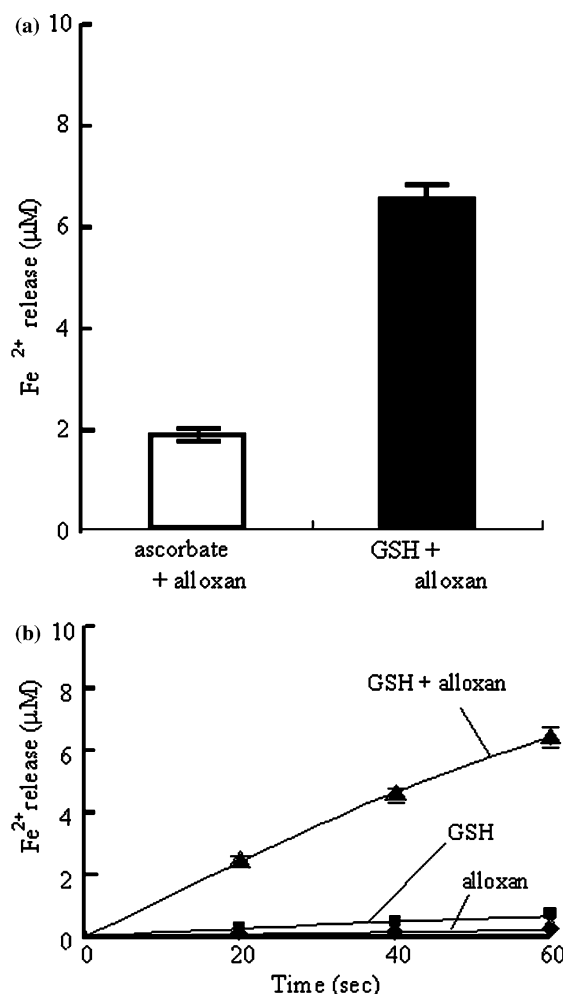
Figure 5. Iron release by ascorbate or GSH in the presence of alloxan. (a) Ferritin (10 μmol as Fe) was incubated with ascorbate (1 mM) or GSH (1 mM) in the presence of alloxan (1 mM). (b) Reactions consisted of 1 mM GSH, 1 mM alloxan, 1 mM BPT in PBS, pH 7.4, at 37 °C. The reaction was initiated by the addition of GSH. Other reaction conditions were as described in the legend to Figure 1. Each value represents the mean ± S.D. of three experiments.
